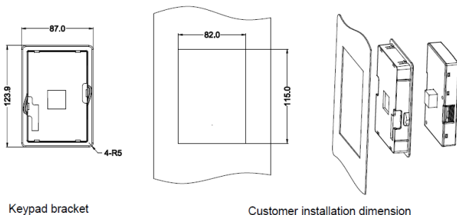
Customer installation dimension
